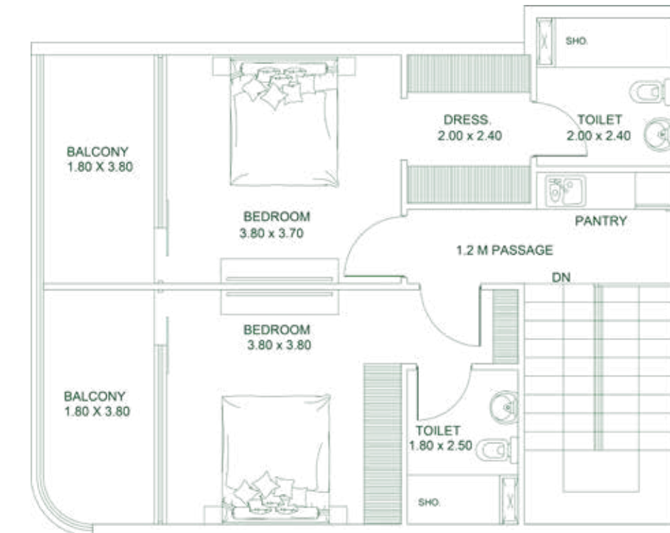
Upper Level
