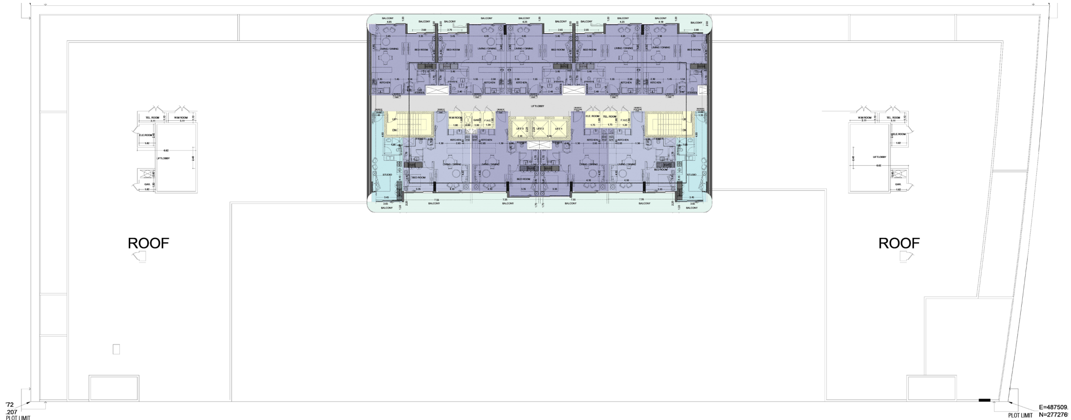
14th TO 18th FLOOR PLAN
