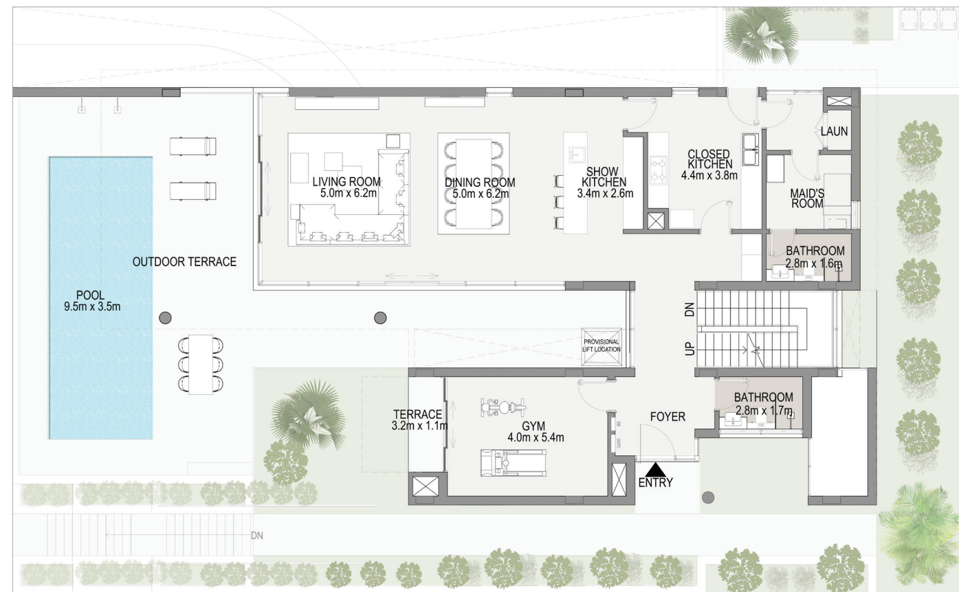
GROUND FLOOR
