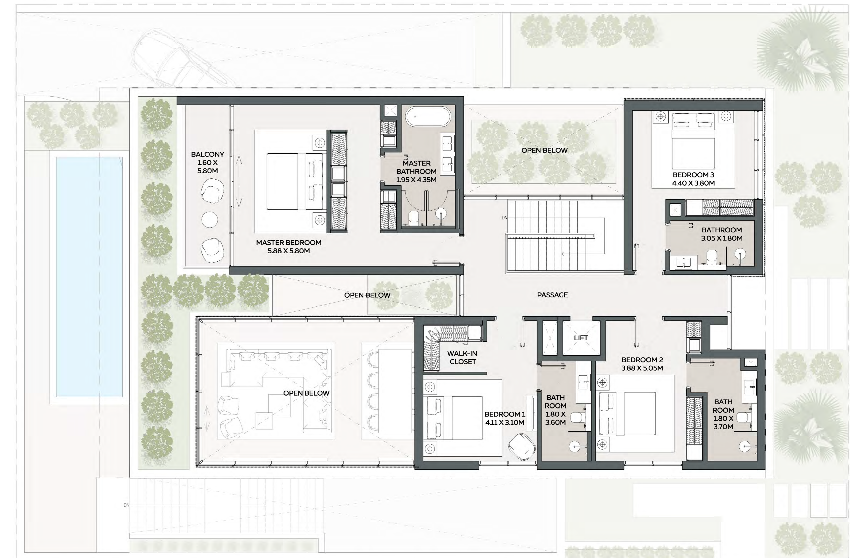
FIRST FLOOR
