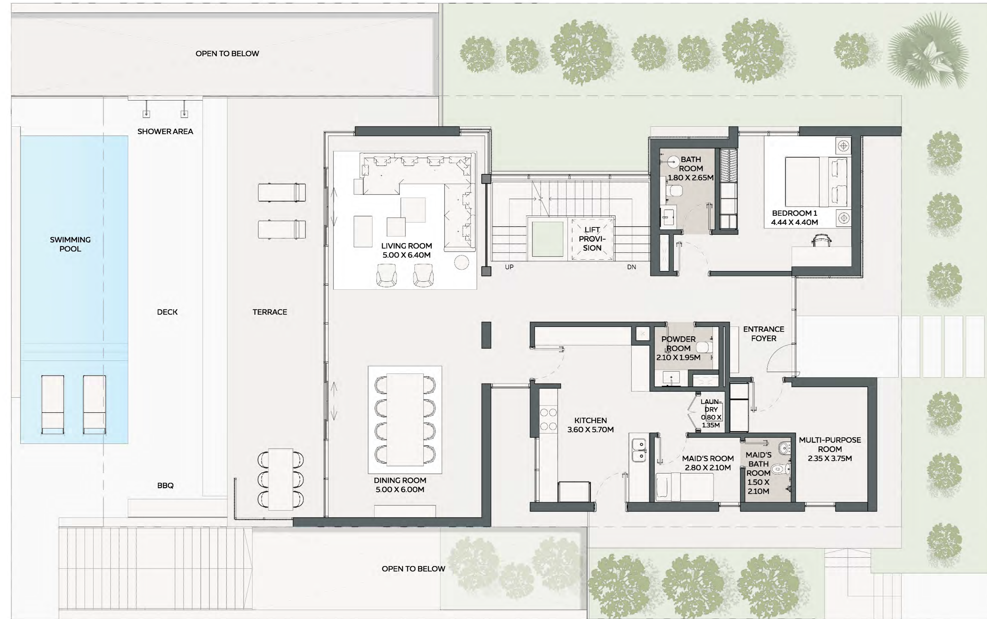
GROUND FLOOR
