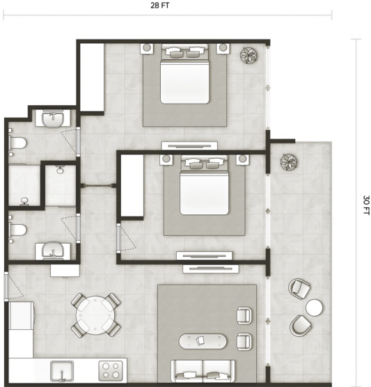
2ND TO 11TH FLOOR
