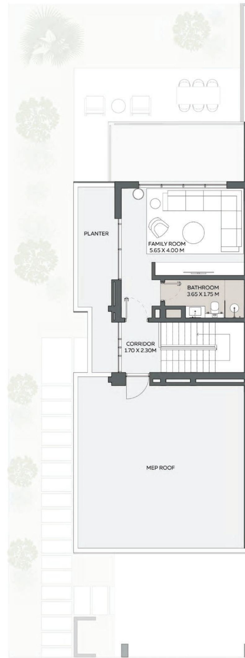
ROOF FLOOR
