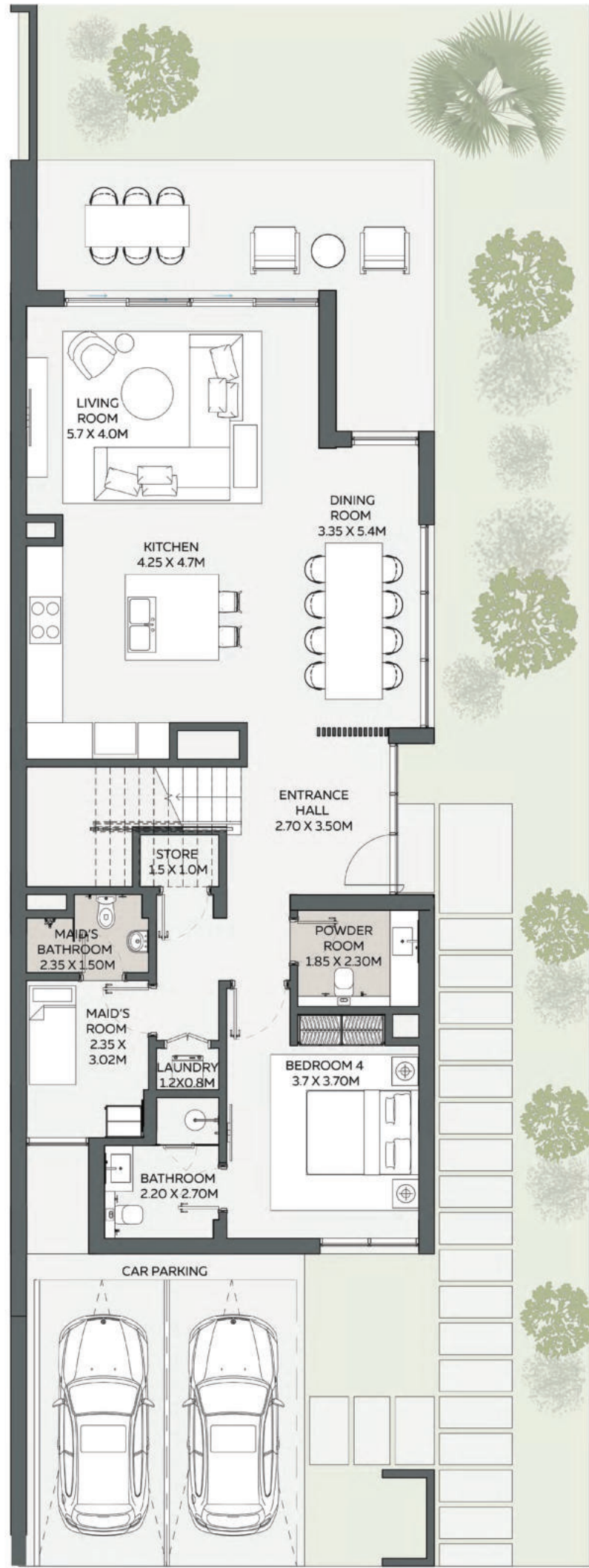
GROUND FLOOR
