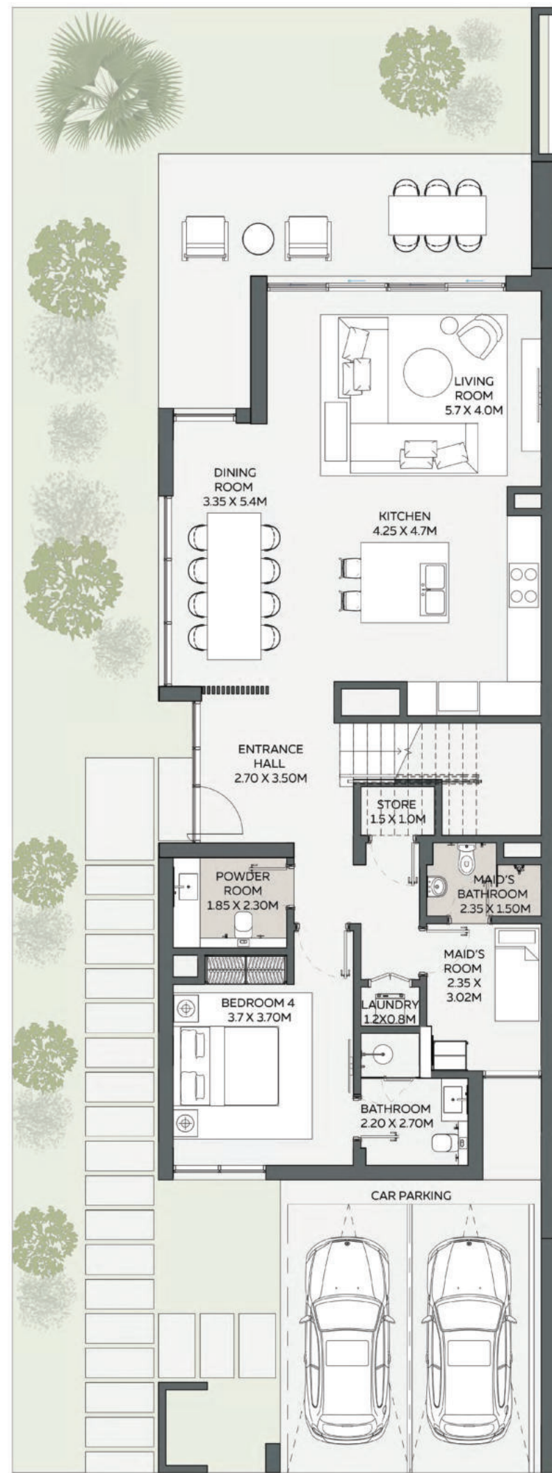
GROUND FLOOR
