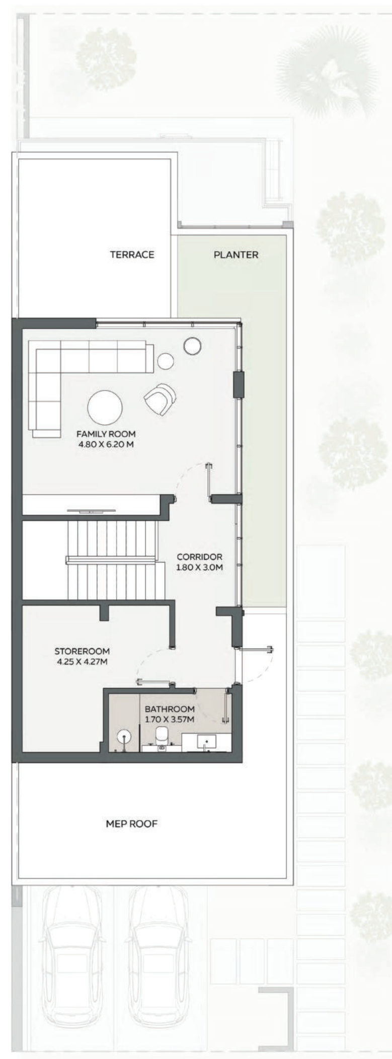
ROOF FLOOR
