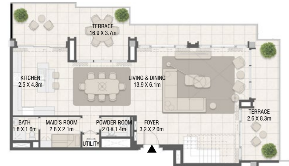
Lower Floor
