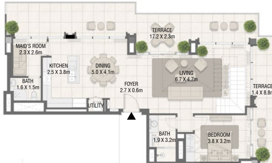
Lower Floor
