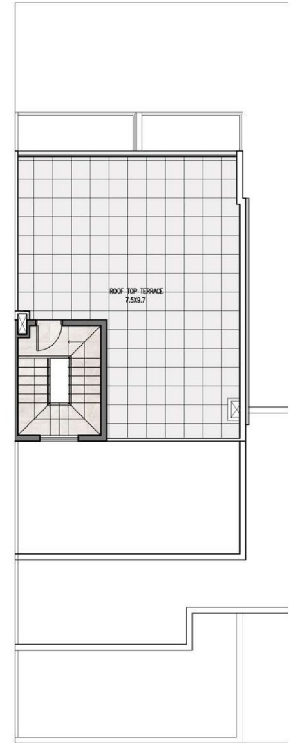
Roof Floor Plan
