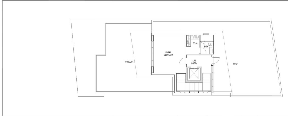
ROOF FLOOR PLAN
