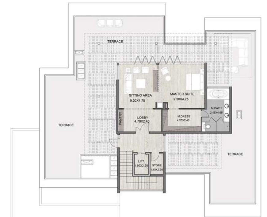
ROOF LEVEL PLAN
