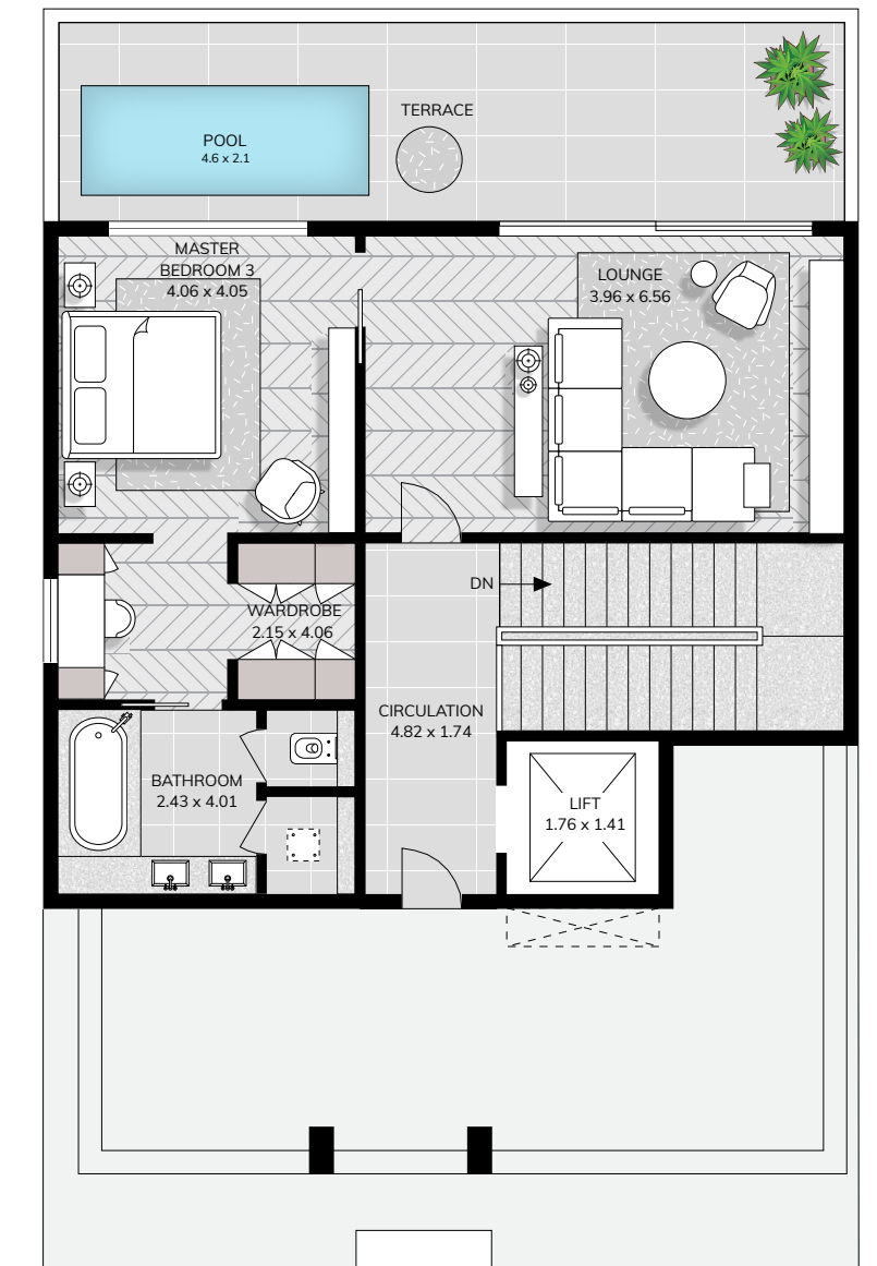
SECOND FLOOR Total Area 135 Sq.m | 1,452 Sq.ft
