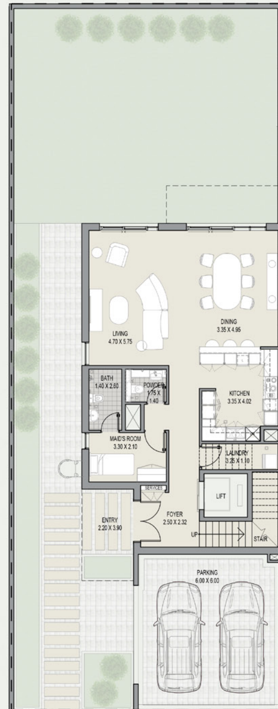
GROUND
