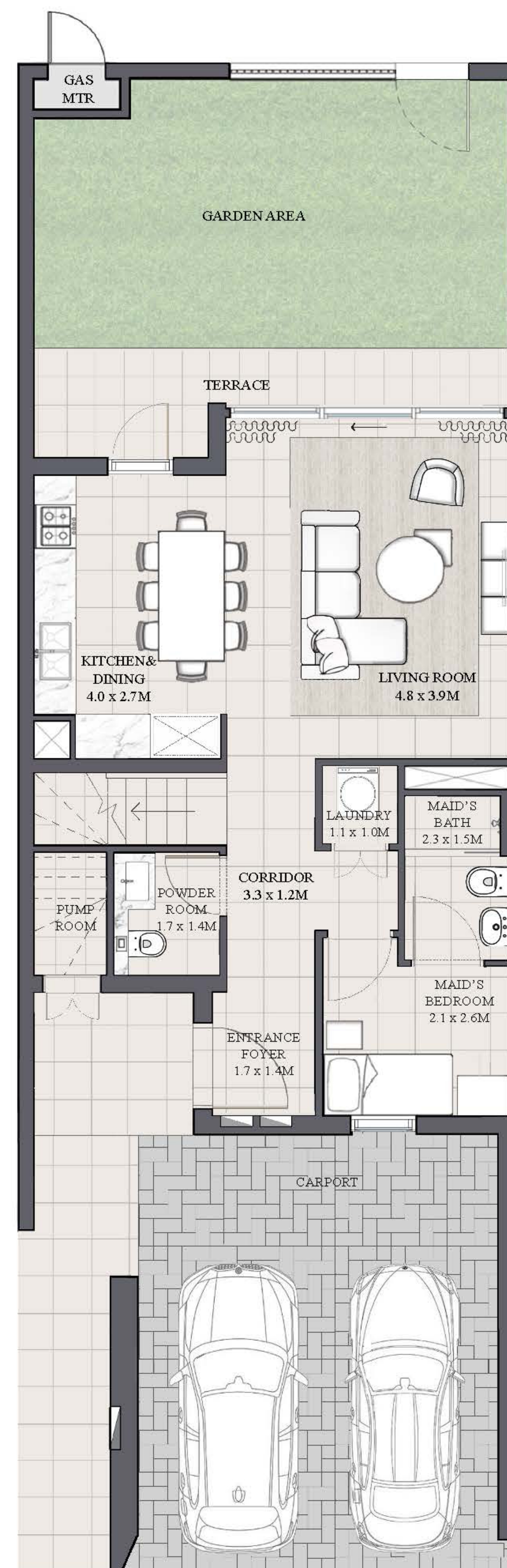
GROUND FLOOR
