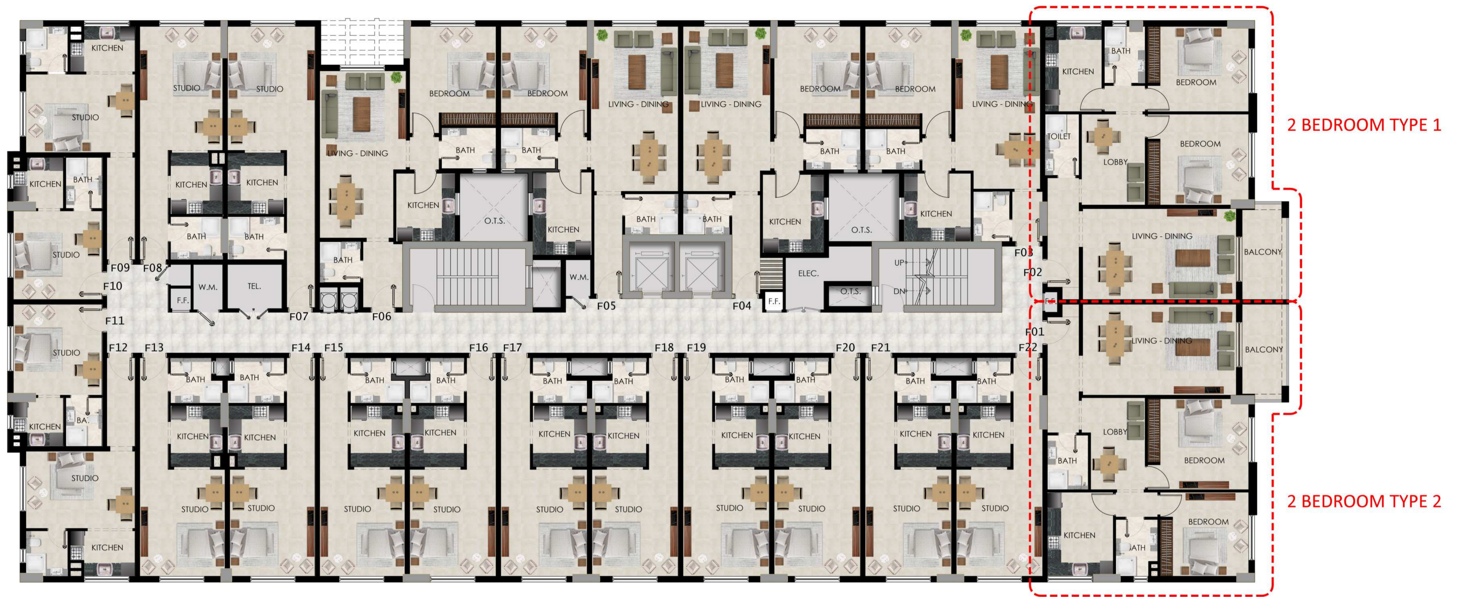
TYPICAL FLOOR PLAN
