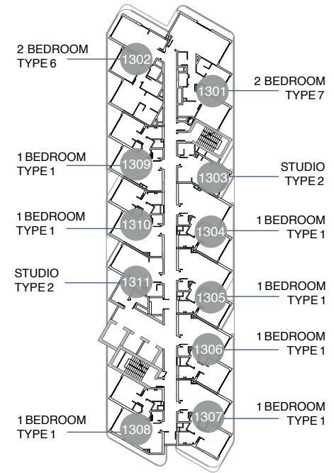
13th FLOOR
