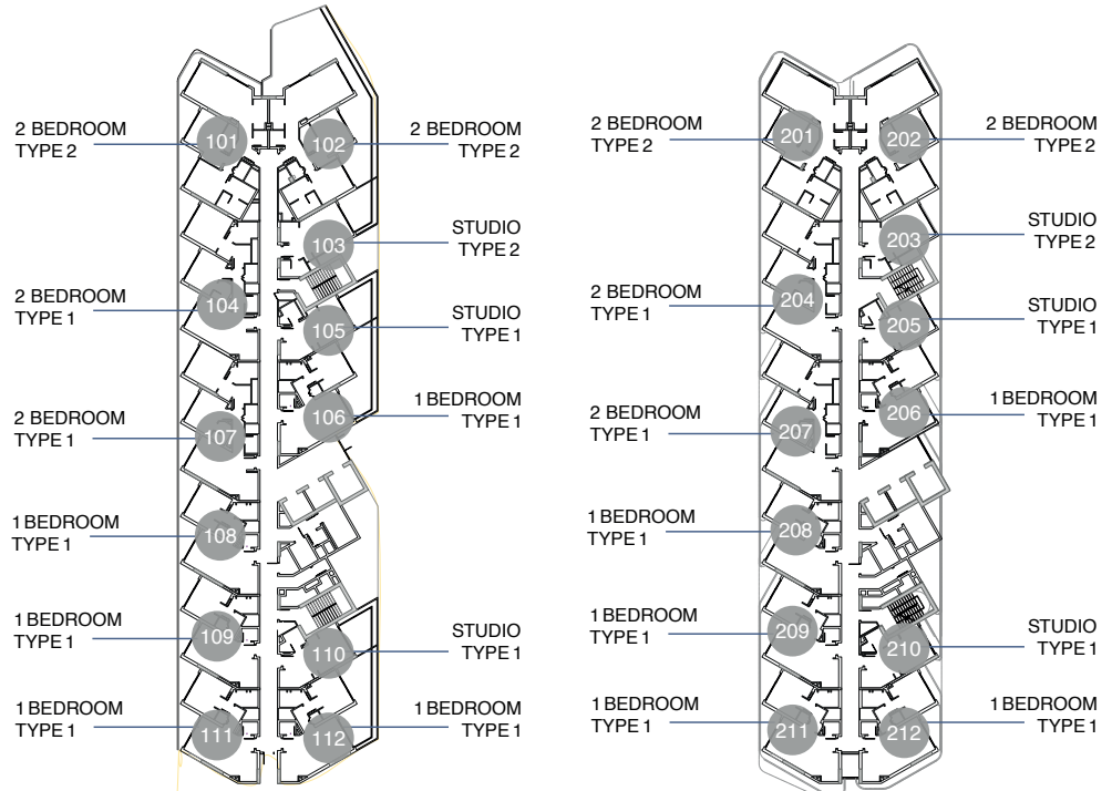
2,4,6th FLOOR
