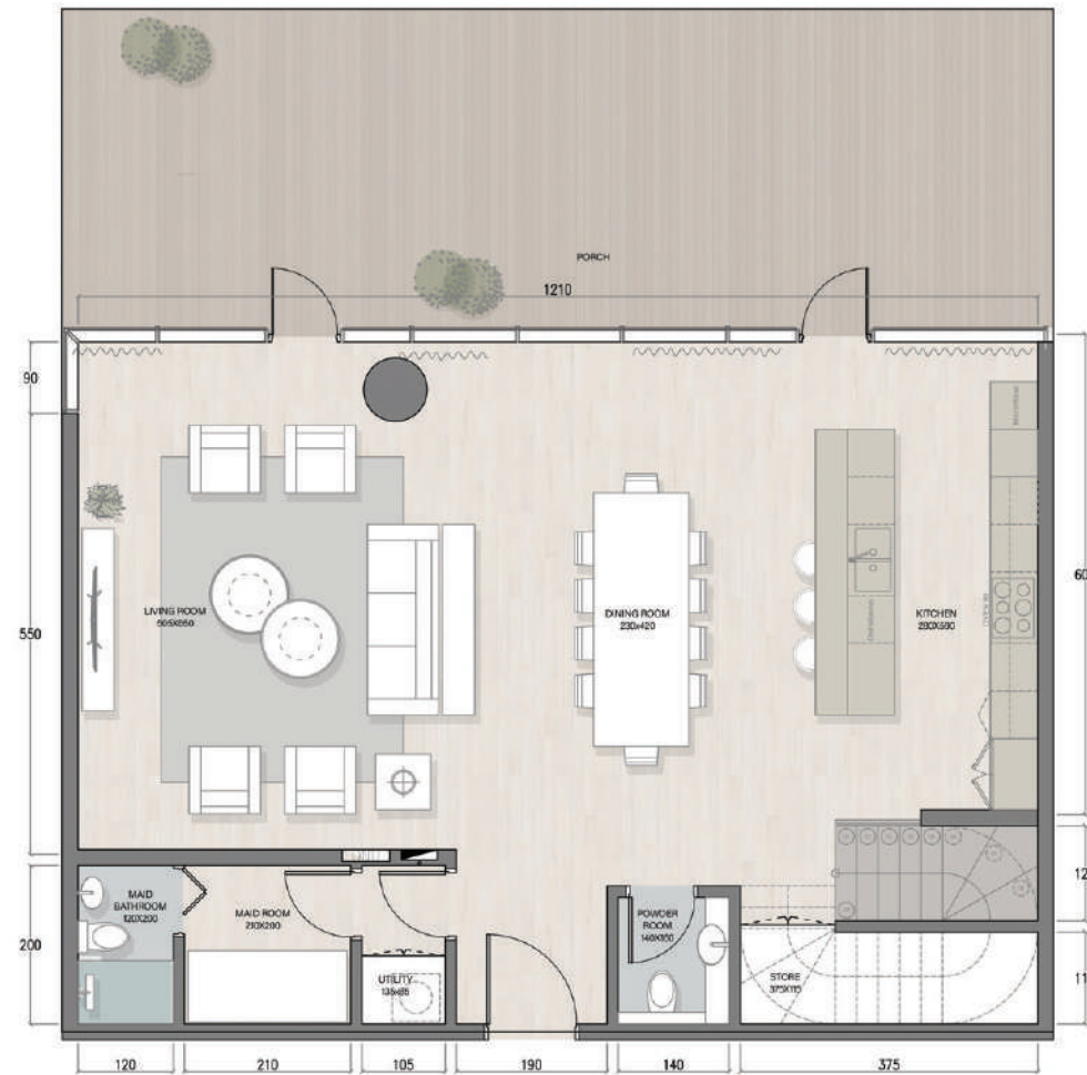
LEVEL 1
