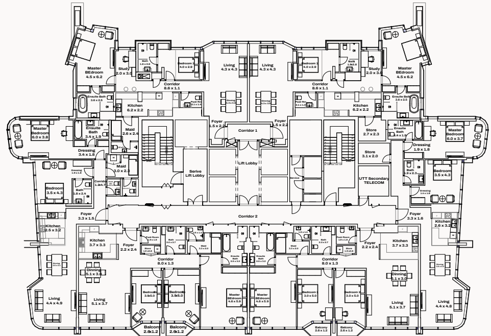
Type 2C6 (1,821.16 sqft) 3 Bedroom + Maid Type 2C7 (1,821.91 sqft) 3 Bedroom + Maid
