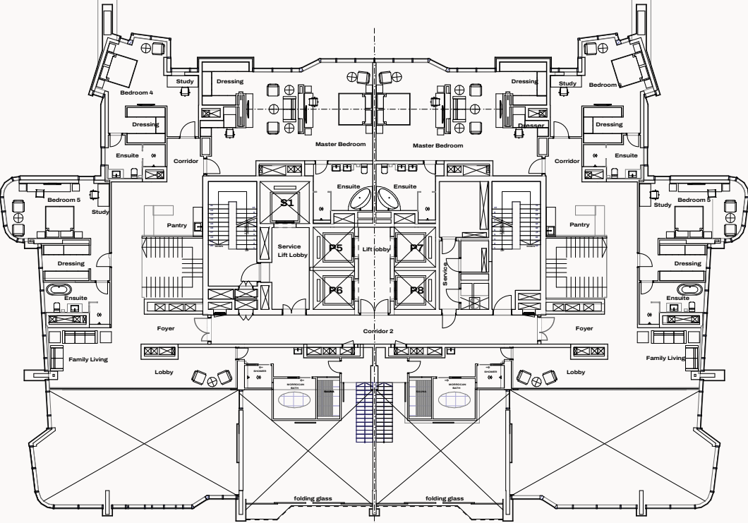
Type P-1 (867.7 sqft) 6 Bedroom Duplex
